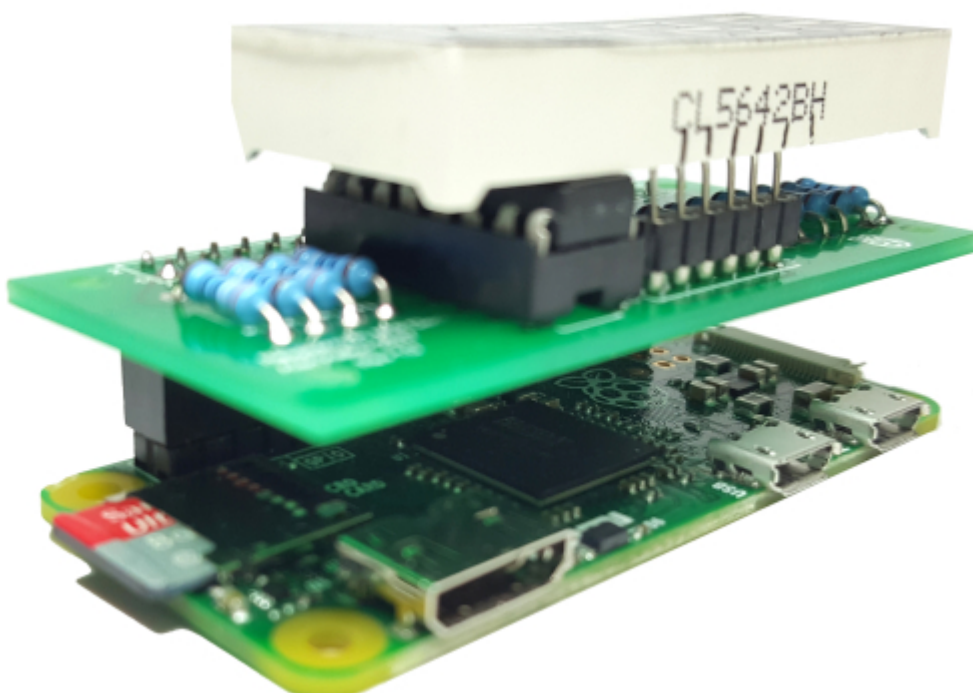
PCB Isometric View with 7 Segment LED attached to Raspberry Pi Zero
