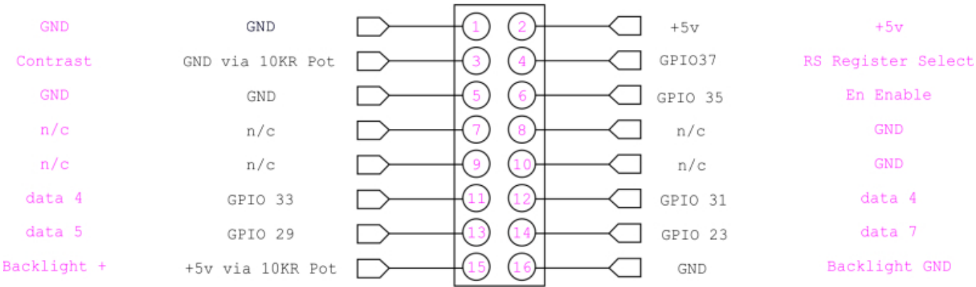
16x2 LCD Interface
